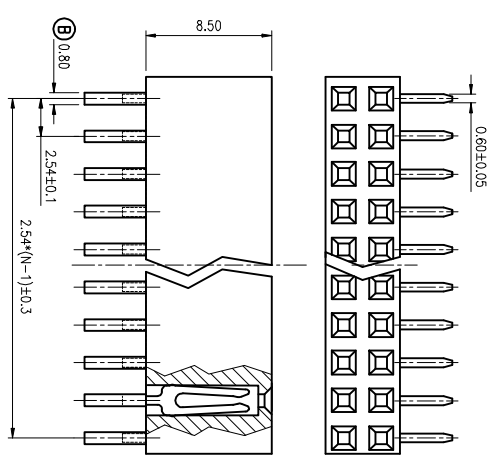
DUAL ROWS N:NUMBER OF CONTACTS/2
